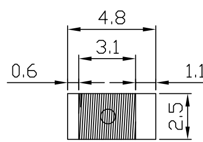
SOLDER PAD Dimension
