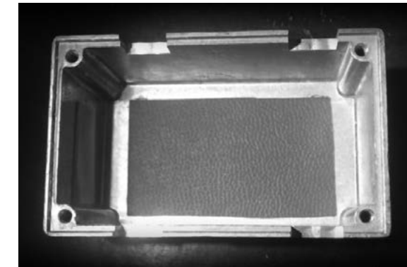
Figure 3. Enclosure with Q-Zorb PN 2238 Installed
