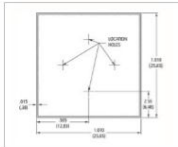
Solder Pad Footprint
