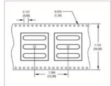
Carrier Tape
