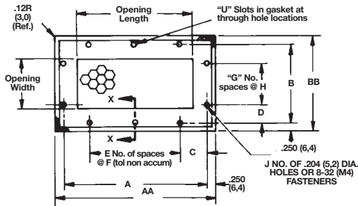
Figure 3. Channel Mount
