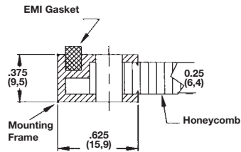
Type 8677
