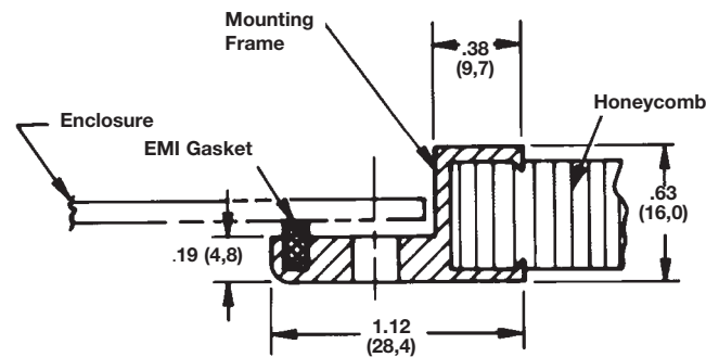
Type 8632
