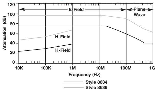
Figure 2. Shielding Effectiveness
