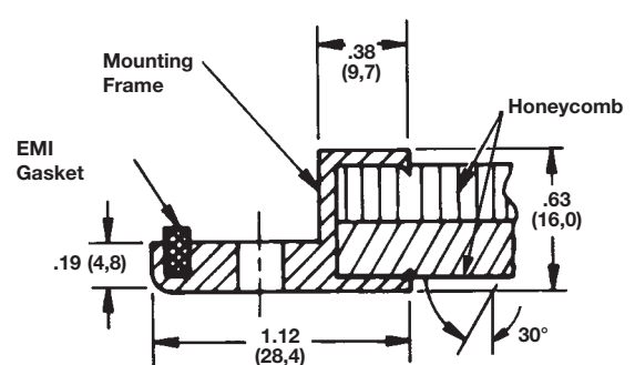
*Type 8633 - Drip-Proof
