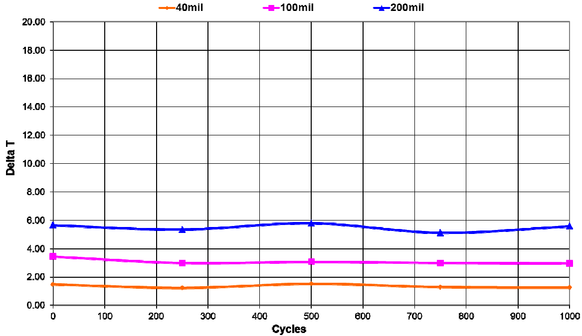
Tflex HD90000 Delta Temperature over 1000 cycles of -50°C to 200°C
