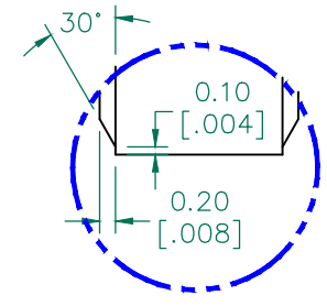
CHAMFER DETAIL A (10:1)
