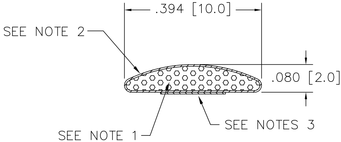
PROFILE DETAIL
